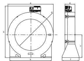
MRCDB30... + CTBC120(P)/CTBC210(P)
