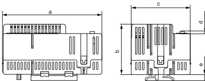
MRCDB30...
